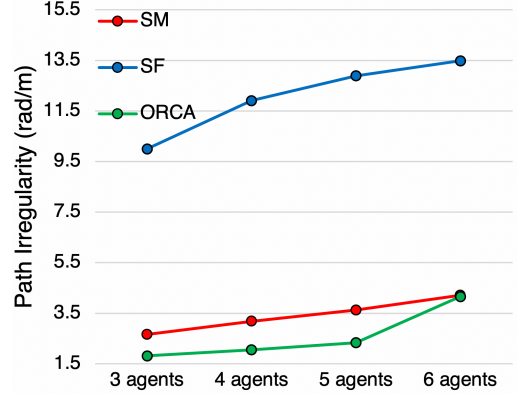
(b) Path Irregularity per agent for each scenario class.
